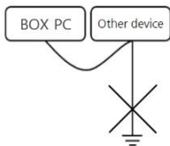
③ Common grounding : Prohibited
